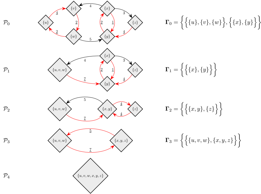
FIGURE 2. Aggregation of states in a CLE decomposition/Edmonds' algorithm. This diagram illustrates cyclic decomposition, moving step by step from \mathcal{P}_0 to \mathcal{P}_4 . The cost function C(\cdot, \cdot) is given by edge weights, with missing edges denoting transitions with infinite cost. The values of C(\cdot, \cdot) on the initial partition \mathcal{P}_0 are assumed. Costs for partitions \mathcal{P}_\ell , \ell > 0 , are calculated as described in the text. Least cost transitions are denoted by an underlined cost and a red arrow, so that a subset of elements in a partition is a cycle if is the vertex set for a (graphical) simple cycle of such edges in the diagram. At each step, one simple cycle is consolidated. For example, in moving from \mathcal{P}_0 to \mathcal{P}_1 , cycle \{\{u\}, \{v\}, \{w\}\} \subset \mathcal{P}_0 is consolidated to form \{u, v, w\} \in \mathcal{P}_1 , with the costs of transitions to and from \{u, v, w\} given by expressions (6) and (7) in the text. For example, C(\{u, v, w\}, \{y\}) = \min\{4 - 4 + \infty, 4 - 2 + \infty, 4 - 2 + 5\} = 7 .
