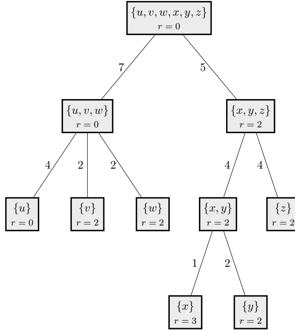
FIGURE 4. The tree structure of decompositions. The tree structure of the decomposition considered in Figure 2. Edges connect composites to their pieces below them in the diagram. Edge weights give \underline{C}(\cdot) for the composite at the lower end of the edge in question. For each composite \alpha , we give r_\alpha which measures the order of magnitude of the probability placed on \alpha by the invariant measure. These are calculated using the values of \underline{C}(\cdot) . For example, \{x, y\} has r_{\{x,y\}} = 2 , therefore by Lemma 3.1, one of its pieces has r = 2 and none have r < 2 . As \underline{C}(\{x\}) = 1 < 2 = \underline{C}(\{y\}) and Lemma 2.1 states that \underline{C}(\{x\}) + r_{\{x\}} = \underline{C}(\{y\}) + r_{\{y\}} , it must be that r_{\{x\}} = 3 and r_{\{y\}} = 2 .
