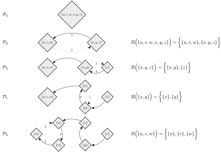
FIGURE 3. Disaggregation of states under Edmonds' algorithm. This diagram illustrates disaggregation and the construction of a spanning tree under Edmonds' algorithm, moving step by step from \mathcal{P}_4 to \mathcal{P}_0 . At each step a composite is expanded into the cycle that formed it during the aggregation phase. For example, \{x, y, z\} \in \mathcal{P}_3 is expanded to \{\{x, y\}, \{z\}\} \subset \mathcal{P}_2 and edges from \{x, y\} to \{z\} and from \{z\} to \{x, y\} are added. Next, edges to or from the composite that is expanded are assigned to the elements of the cycle that solved (6) or (7) when the cycle was consolidated during the aggregation phase. For example, the edge from \{x, y, z\} to \{u, v, w\} is replaced by an edge from \{x, y\} to \{u, v, w\} . Finally, an edge in the expanded cycle is deleted (denoted by a dotted line in the diagram). If the expanded composite was not the root of the tree at the previous step (e.g. \{x, y, z\} in \mathcal{P}_3 ), then the element of the cycle with an outgoing edge to outside of the cycle (e.g. \{x, y\} in \{\{x, y\}, \{z\}\} ) has its outgoing edge within the cycle deleted (e.g. the edge from \{x, y\} to \{z\} ). If the expanded composite was the root of the tree at the previous step (e.g. \{u, v, w\} in \mathcal{P}_1 ), then the element of the cycle with the highest least cost transition (e.g. \{u\} in \{\{u\}, \{v\}, \{w\}\} ) has its outgoing edge deleted (e.g. the edge from \{u\} to \{v\} ).
