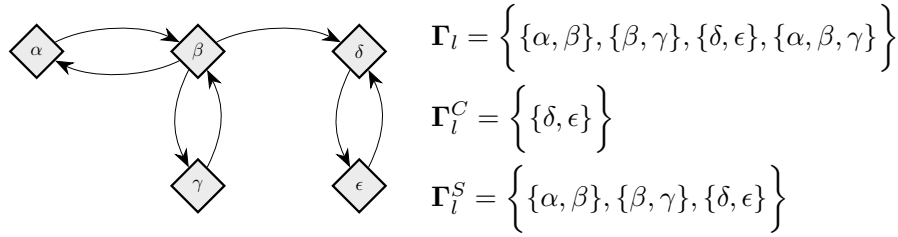
FIGURE 1. Cycles. For given least cost correspondence, the set of cycles, closed cycles and simple cycles.
