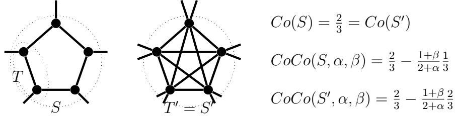
Figure 6: Let \Gamma = (V, E) contain the subgraphs on vertex sets S and S' shown above. Let \Omega be the set of cliques , sets T \subseteq V such that every member of T is a neighbor of every other member of T . If \beta > -1 , then values for cohesion and coalitional cohesion are as given above. Note that although S and S' are equally cohesive, more integrated coalitions are possible within S' than within S ( d(i, T')/d(i) = 2/3 for i \in T' , whereas d(i, T)/d(i) = 1/3 for i \in T ). Consequently, S' is less coalitionally cohesive than S . If \beta \leq -1 , then coalitional cohesion equals cohesion as discussed in the text.
