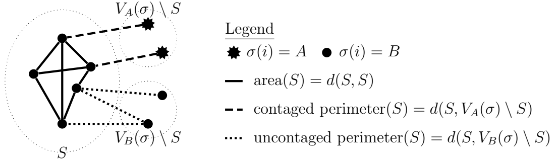
Figure 2: Illustration of graph theoretic properties. Stars and circles represent players playing A and B respectively. Lines (solid, dashed, dotted) represent edges between neighboring players. In this example, d(S, S) = 7 , d(S, V_A(\sigma) \setminus S) = 2 and d(S, V_B(\sigma) \setminus S) = 3 .
