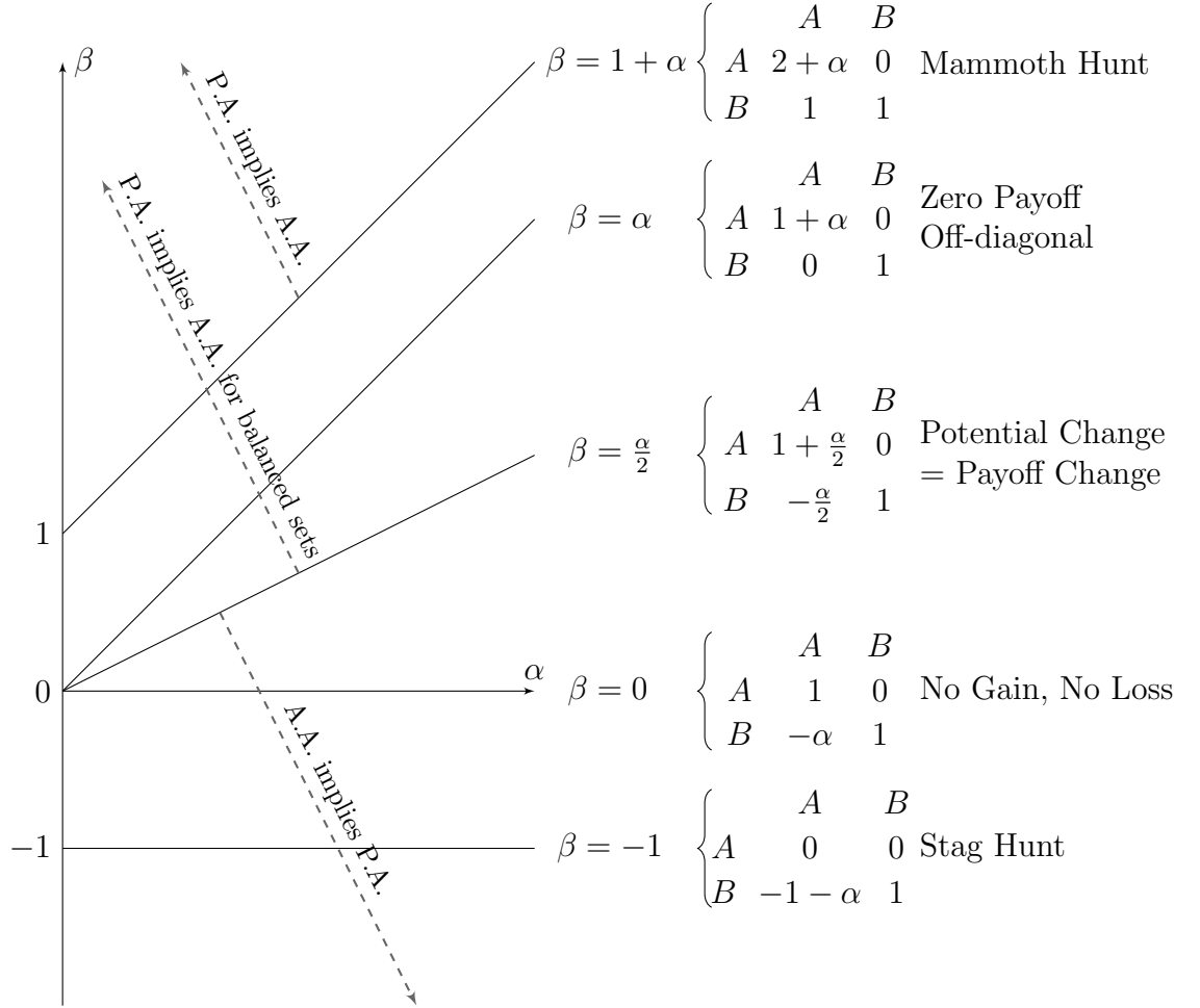
Figure 4: Propositions 1, 2, 3 illustrated in \alpha - \beta space. The ordinal ranking of payoffs in the game changes at \beta = 1 + \alpha , \beta = \alpha , \beta = 0 , \beta = -1 . At \beta = \alpha/2 , if \sigma_S changes, then the consequent change in the sum of the payoffs of players in S exactly equals the change in potential.
